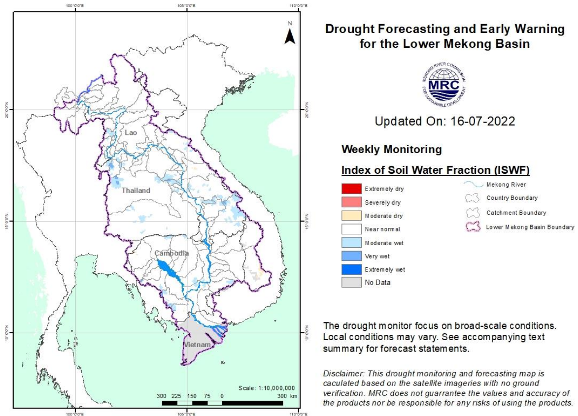
Figure 16. Index of Soil Water Fraction from 10 to 16 July 2022.
