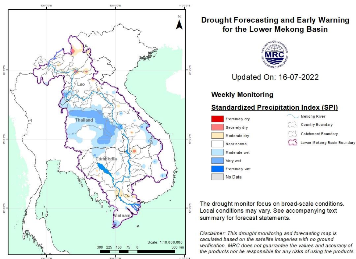
Figure 15. Weekly standardized precipitation index from 10 to 16 July 2022.
