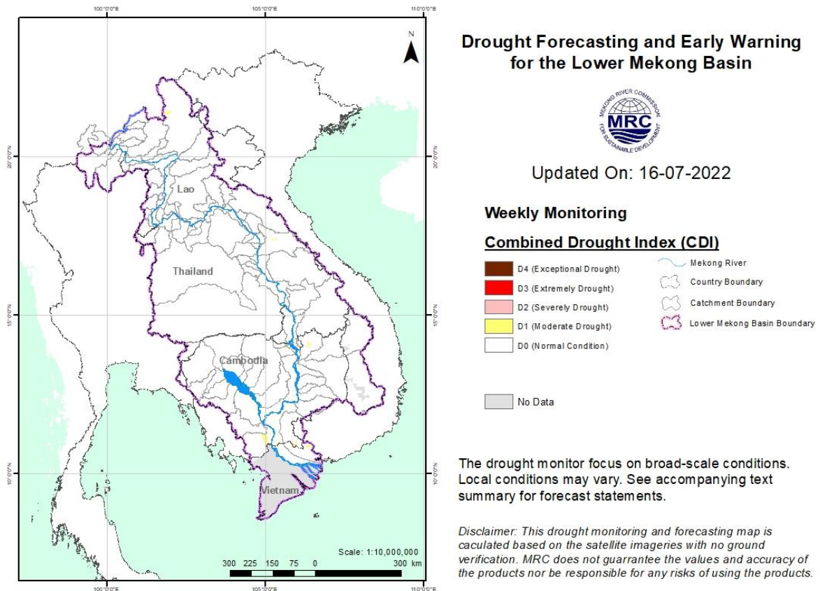
Figure 17. Weekly Combined Drought Index from 10 to 16 July 2022.
