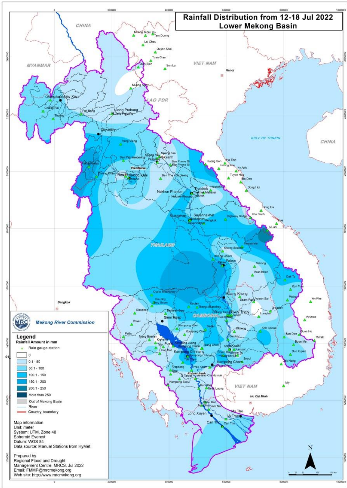
Figure 5. Weekly rainfall distribution over the LMB during 12-18 July 2022.
