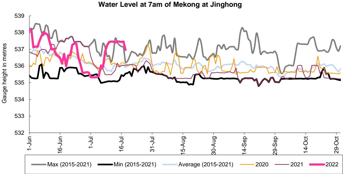
Figure 7. Water level at the Jinghong hydrological station up to 18 July 2022.
