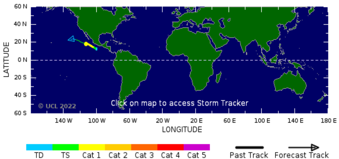
Figure 3. A tropical depression risk observed on 18 July 2022.
